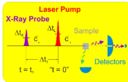
Figure 1: A schematic of a pump-probe-experiment [?].
