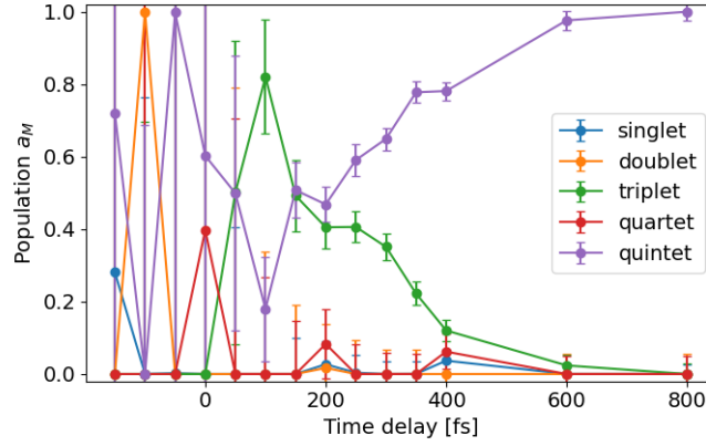
Figure 9: The population curves of the different spin states plotted against the time delay of the optical laser in femtoseconds.
